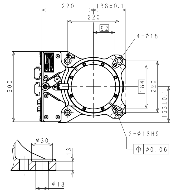
Installation Dimensions
